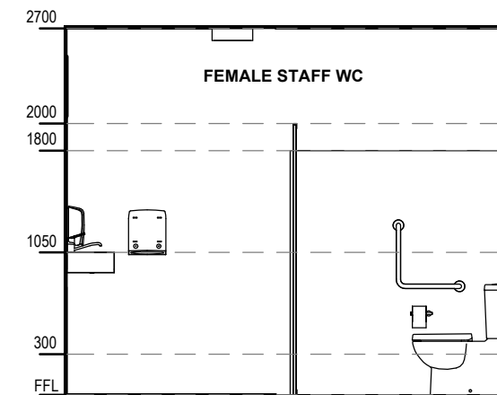
7 FEMALE STAFF WC ELE 7 SCALE: 1 : 50
