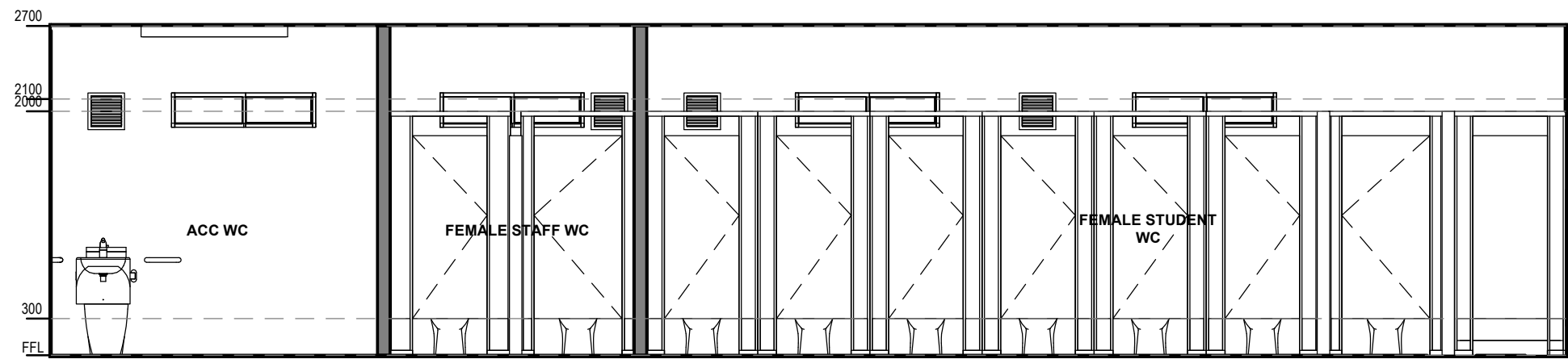
1 ACC WC, FEMALE STAFF & ST WC ELEVATION SCALE: 1 : 50
