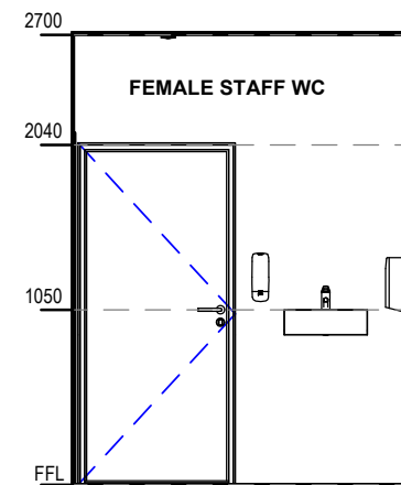
6 FEMALE STAFF WC - ELE 6 SCALE: 1 : 50
